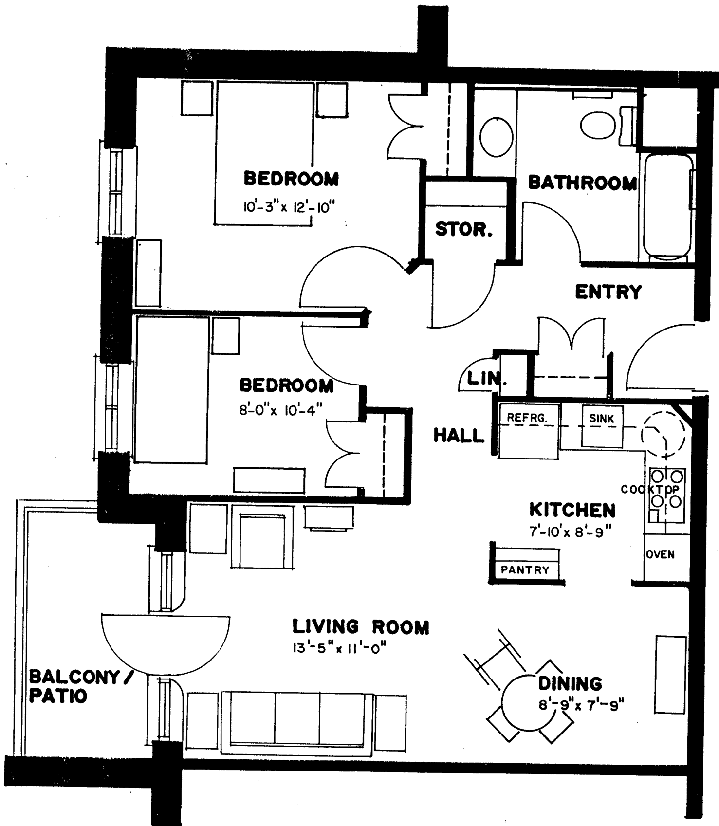
TYPICAL TWO BEDROOM · TYPE 'B' UNIT CONVERTIBLE / HANDICAPPED
